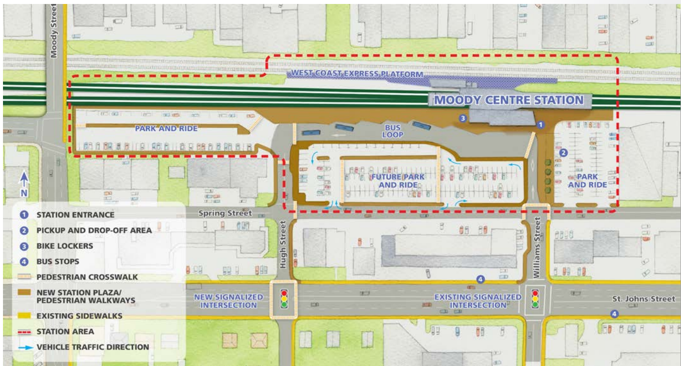
Site context plan for completed Moody Centre Station
